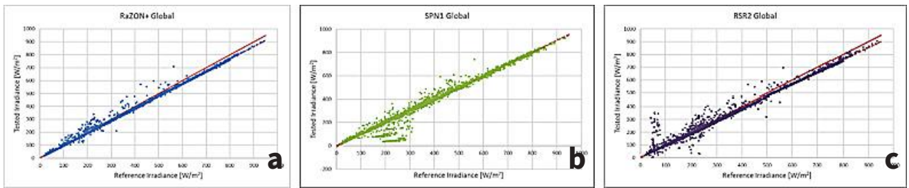
Figure 6 GHI measurements plotted with on the x-axis the reference irradiance and on the y-axis the (a) RaZON + , (b) SPN1, and (c) RSR2 data. The solid red line is y=x and the dashed red line is the fit of the measurement points.
