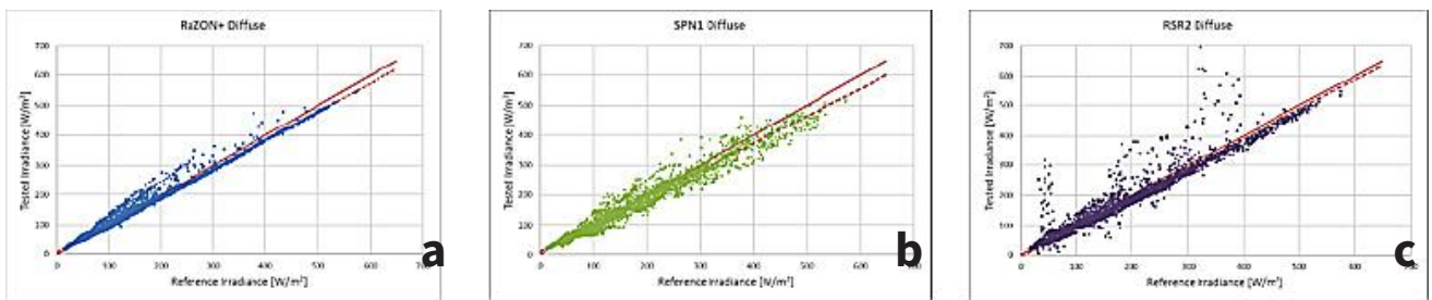
Figure 7 DHI measurements plotted with on the x-axis the reference irradiance and on the y-axis the (a) RaZON + , (b) SPN1, and (c) RSR2 data. The solid red line is y=x and the dashed red line is the fit of the measurement points.
